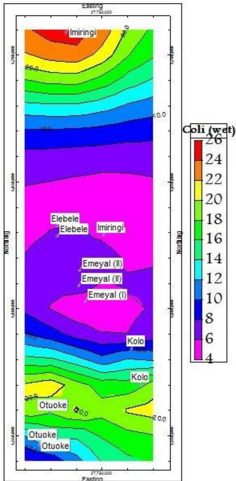
Fig. 3. Coliform concentration in the study area (wet season)
