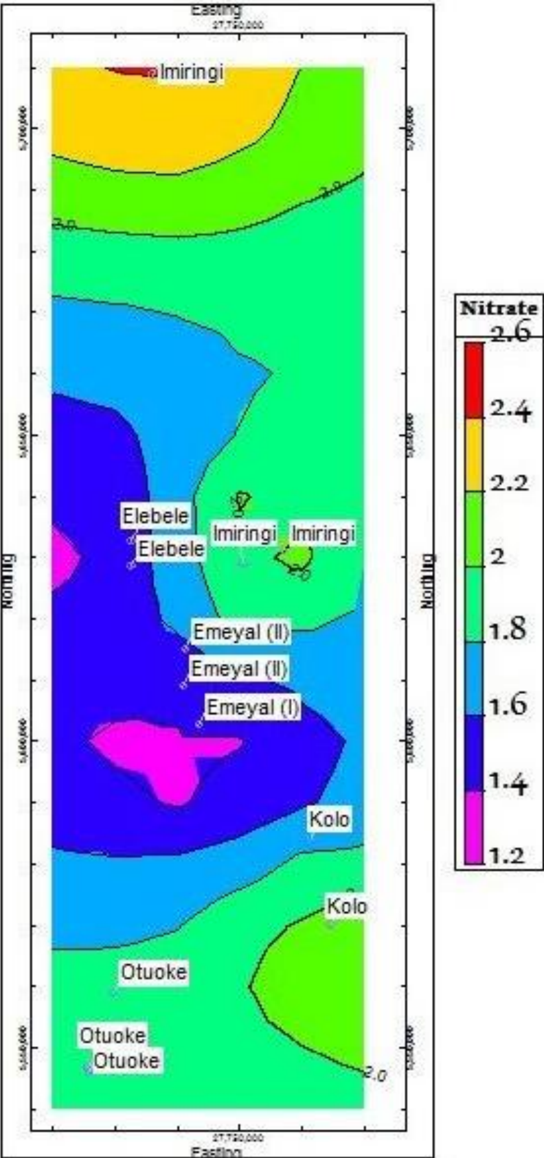
Fig. 10. Nitrate concentration in the study area
