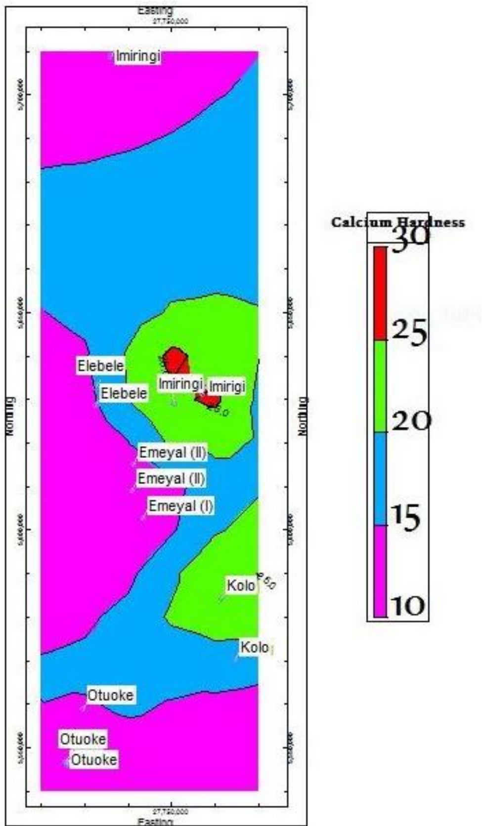
Fig. 15. Calcium hardness concentration in the study area
