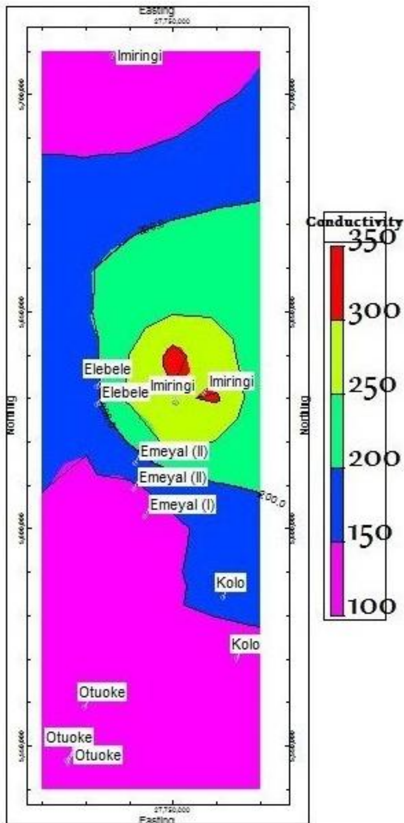
Fig. 7. Conductivity concentration in the study area
