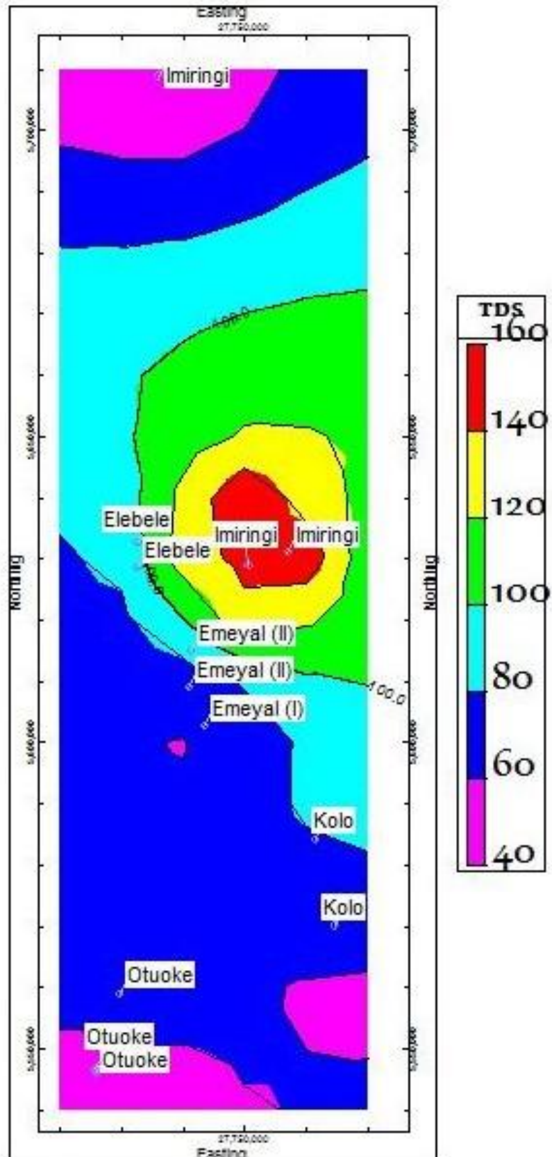
Fig. 12. TDS concentration in the study area
