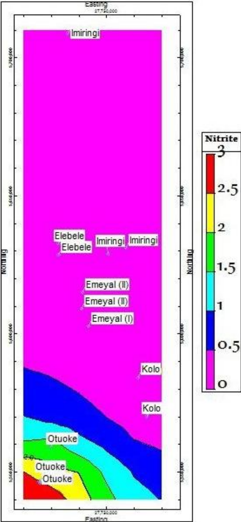
Fig. 11. Nitrite concentration in the study area
