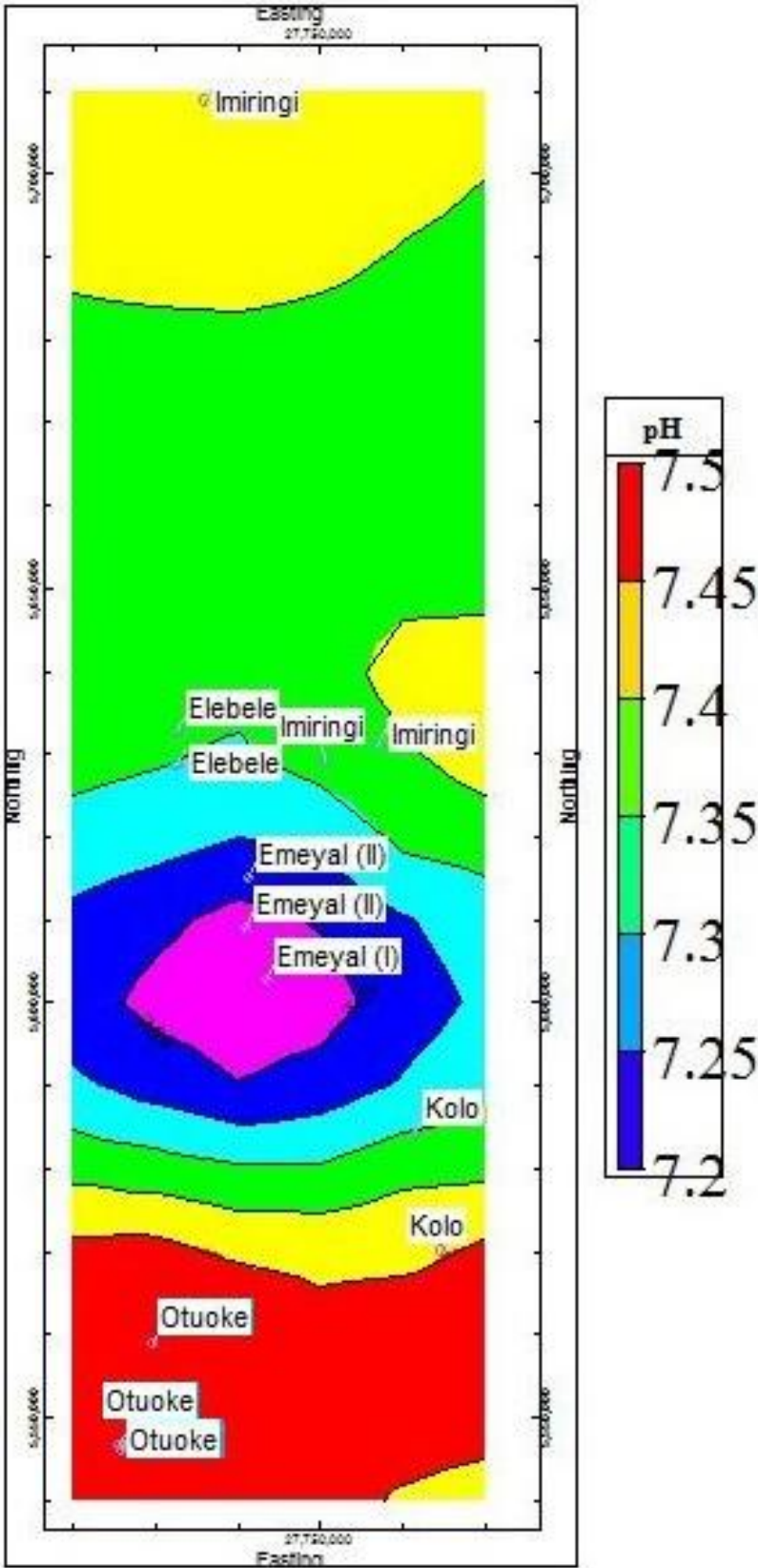
Fig. 5. pH concentration in the study area
