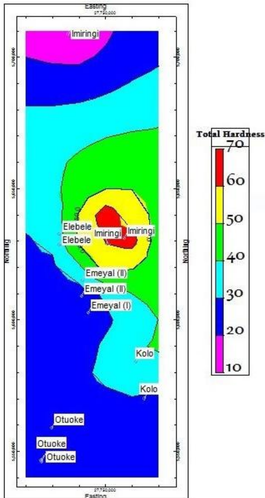
Fig. 14. Total hardness concentration in the study area
