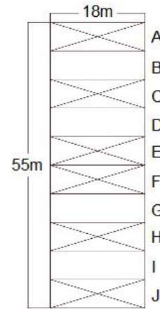
Fig. 3. Bracing scheme for the span of 18 meters (model 6)
