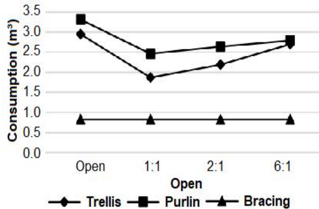
Fig. 7. Graphical representation showing comparative consumption for 12 meters span
