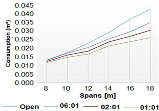
Fig. 4. Graphical representation showing comparative consumption for all spans
