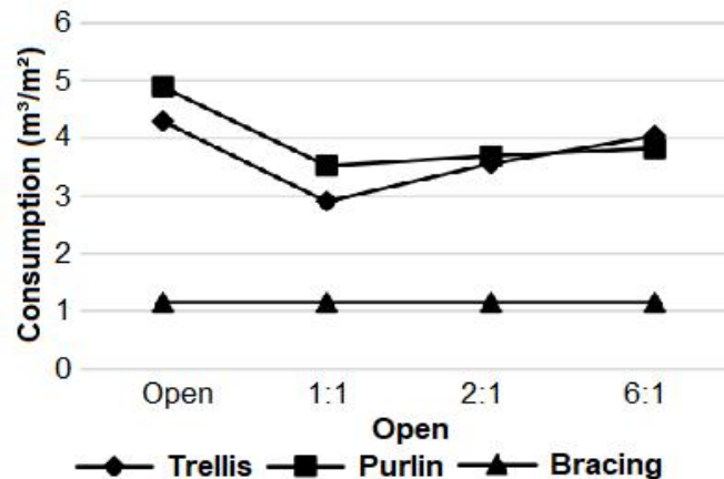
Fig. 8. Graphical representation showing comparative consumption for 14 meters span
