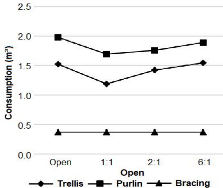
Fig. 6. Graphical representation showing comparative consumption for 10 meters span
