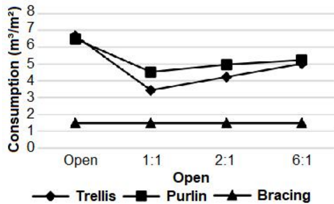
Fig. 9. Graphical representation showing comparative consumption for 16 meters span
