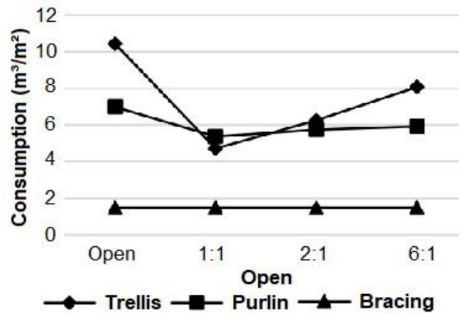
Fig. 10. Graphical representation showing comparative consumption for 18 meters span
