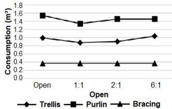
Fig. 5. Graphical representation showing comparative consumption for 8 meters span
