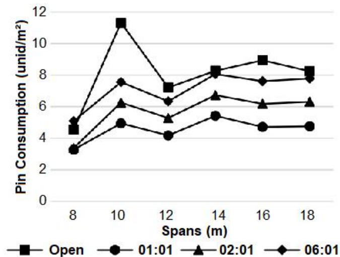
Fig. 11. Graphical representation showing comparative consumption for 18 meters span
