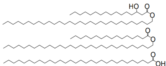
Fig. 11. Main elements of beeswax structure
