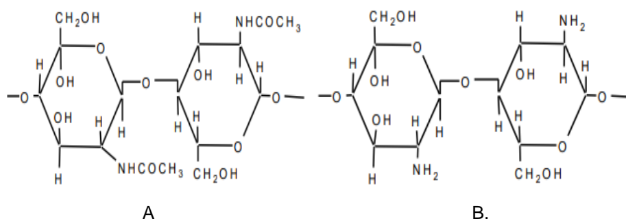
Fig. 8. Chemical structure of chitin (A) and chitosan (B)
