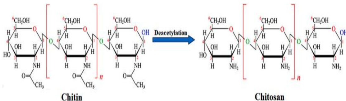
Fig. 9. Chitin molecular deacetylation reaction to chitosan
